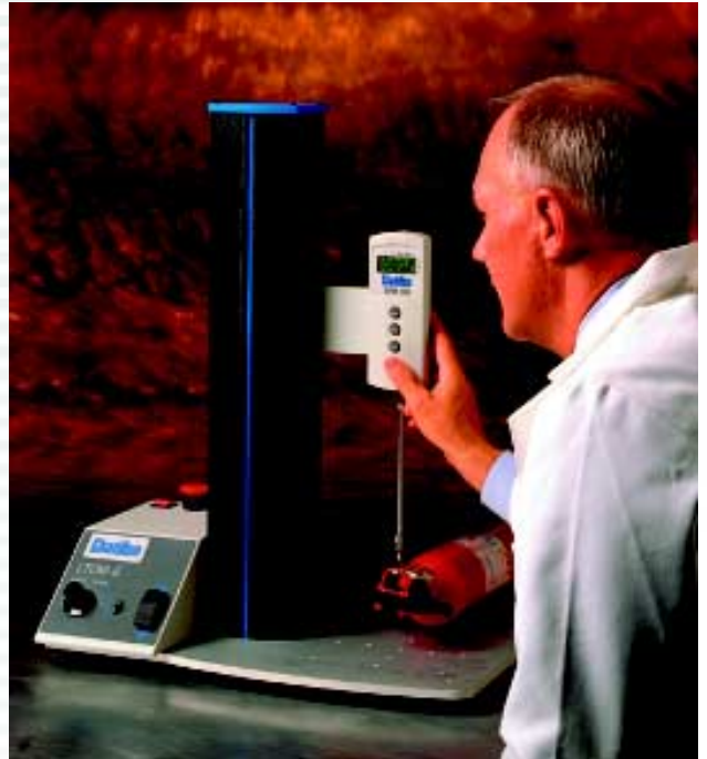
LTCM shown with DFM digital force gauge
