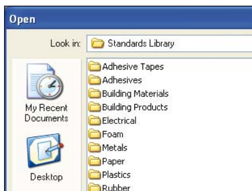
Standards Library
